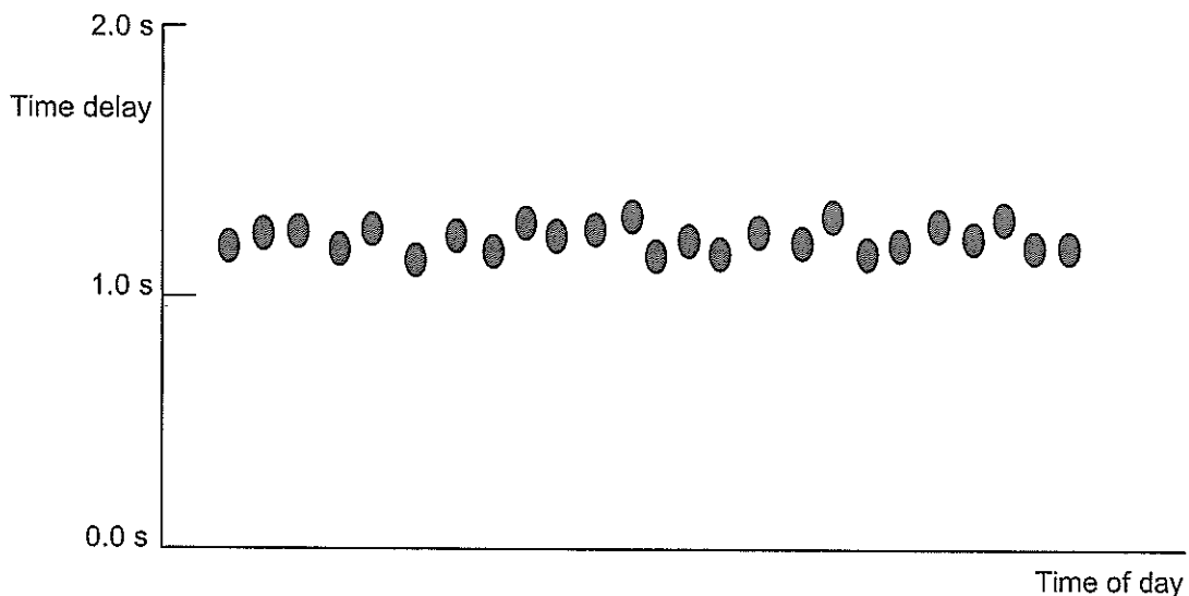
Figure 5: Record of echoes received by an acoustic sounder in Perth.
