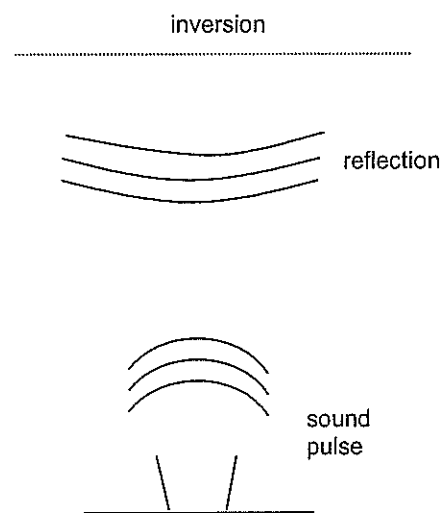
Figure 3 Principle of the acoustic sounder
