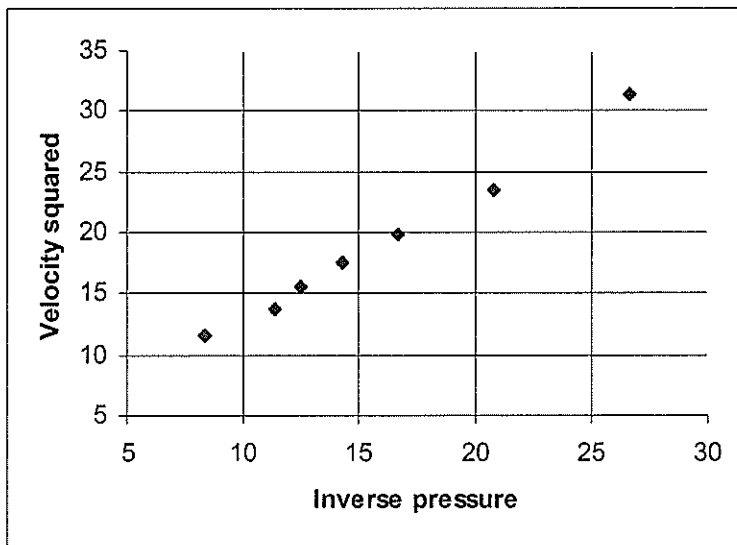
Figure 6: Plot of v^2 vs 1/p .
